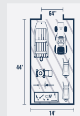
14'x44'
